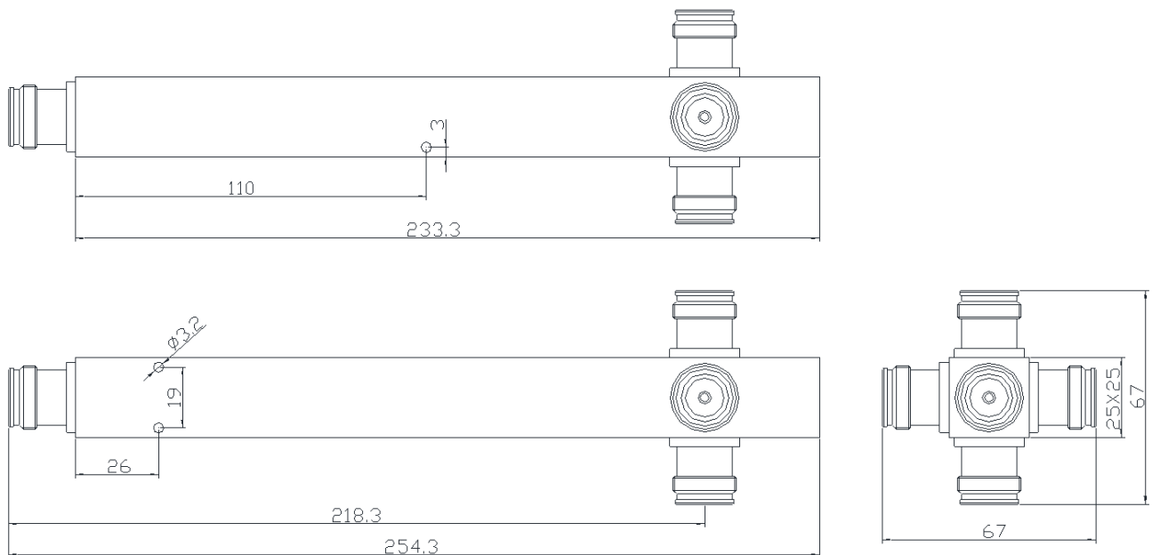
Figure 1 JX-PS-4-4310 front panel layout
